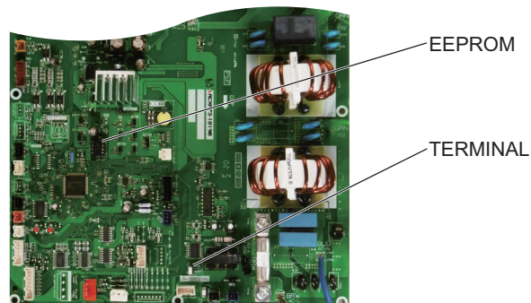
ACXA73-18190 : (U-125PZ2E5, U-140PZ2E5) (for single-phase outdoor unit PCB)
