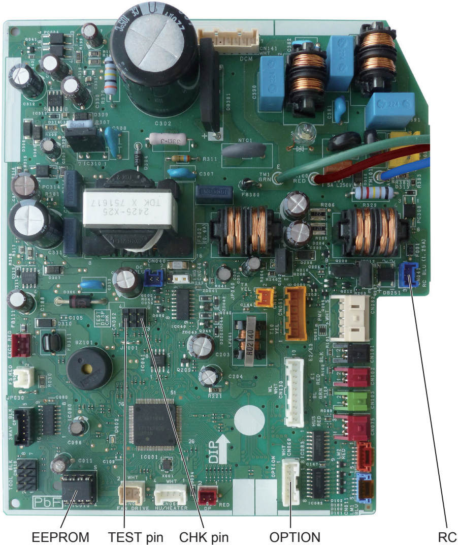
ACXA73C41820 : Wall Mounted Type (Type K2) Indoor Unit Control Board
